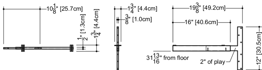
plan view
